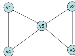
No Hamiltonian Circuit
