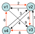
Tour {v1, v2, v3, v4, v1} Distance: 2+6+8+6=22
