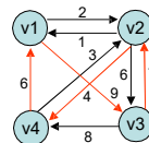
Tour {v1, v3, v2, v4, v1} Distance: 9+7+4+6=26
