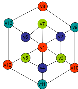
4- color graph with minimum colors
