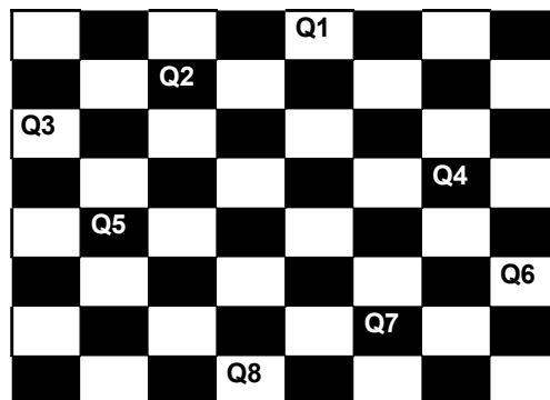
A possible solution of 8-queen problem
